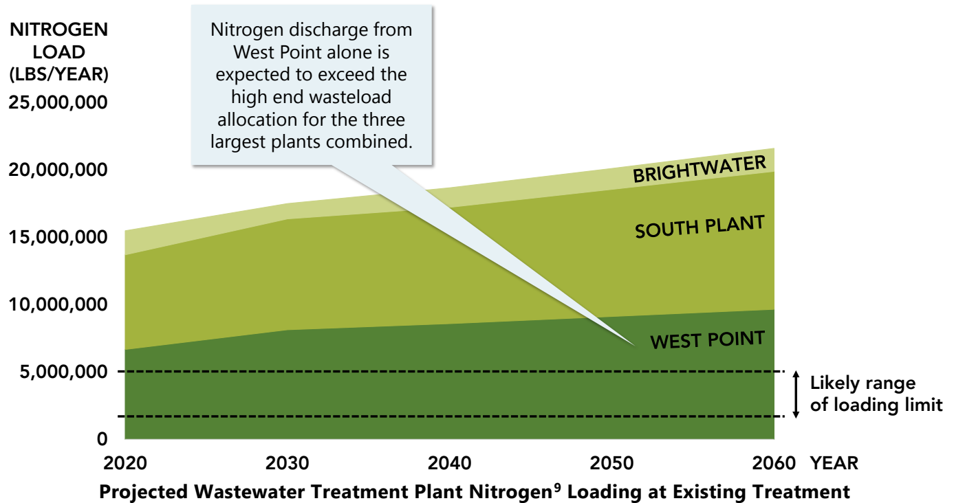
EXHIBIT D: Without significant reductions, King County will not comply with potential future nutrient limits developed by the Department of Ecology.
