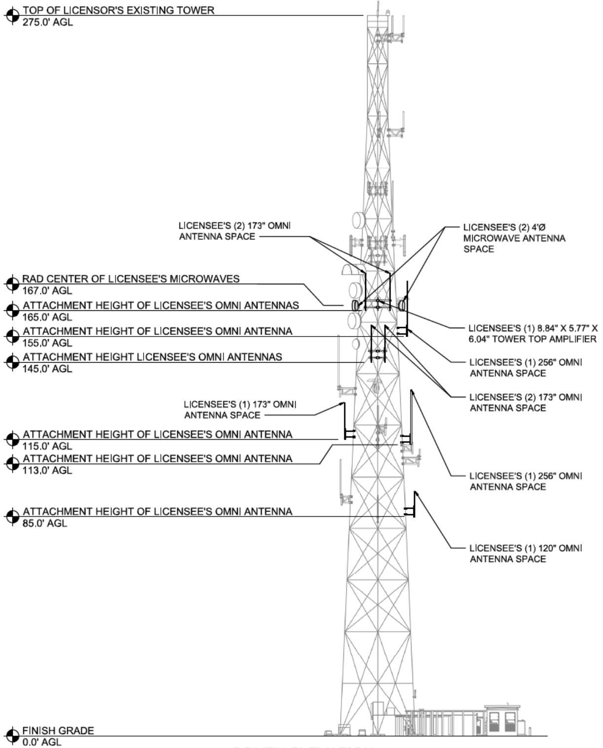
SOUTH ELEVATION
