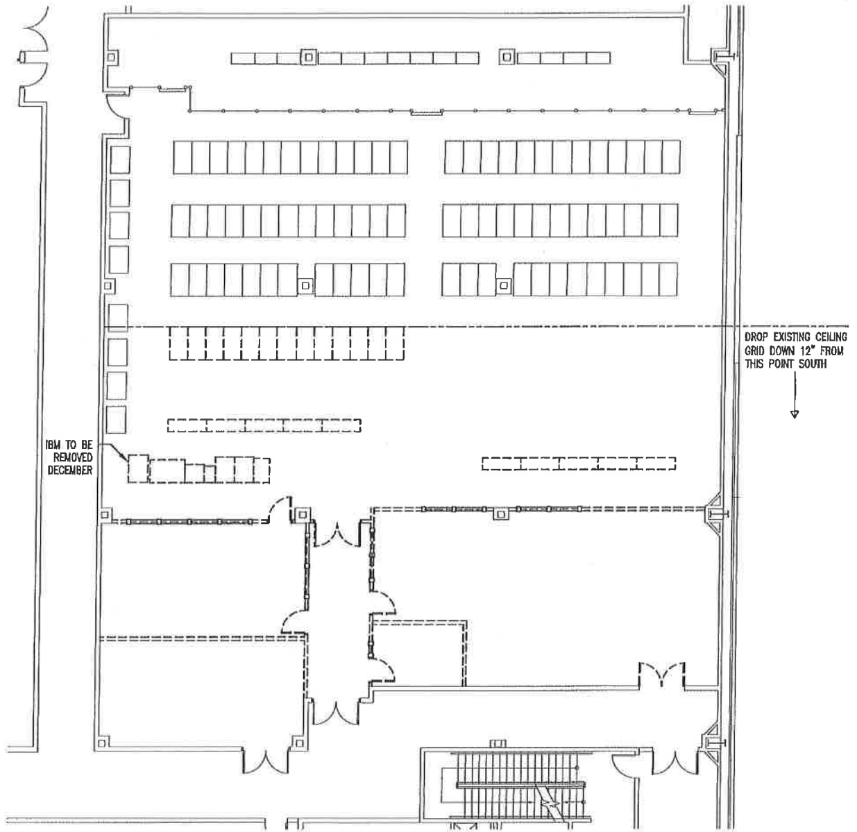
1 SDC52-01 DEMOLITION PLAN SCALE: 1/16" = 1'-0"
