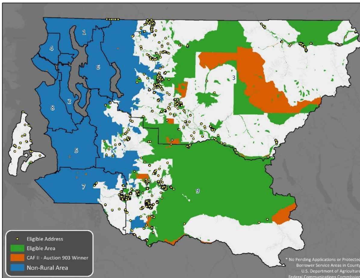
Figure 51: ReConnect-Eligible Addresses
