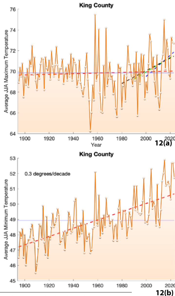
Figures 12(a) and (b). Summer (Jun-Aug, or "JJA") maximum temperatures (top) and minimum temperatures (bottom) for King County from 1895-2023. The linear trend line for the entire period of record is the dashed red line. The blue line is the average for the period of record (1895-2023). Trends in maximum temperature for more recent periods are shown as follows: 1980-2023 (dashed black line), 1990-2023 (dashed green line), and 2000-2023 (dashed blue line). Recent years show more warming in maximum summer temperatures. Figure source: K. Bumbaco, Office of the Washington State Climatologist using NOAA NCEI Climate at a Glance ; accessed February 27, 2024.
