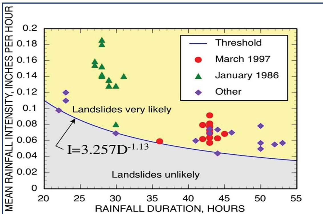
Figure 12-7. Intensity Duration Threshold
