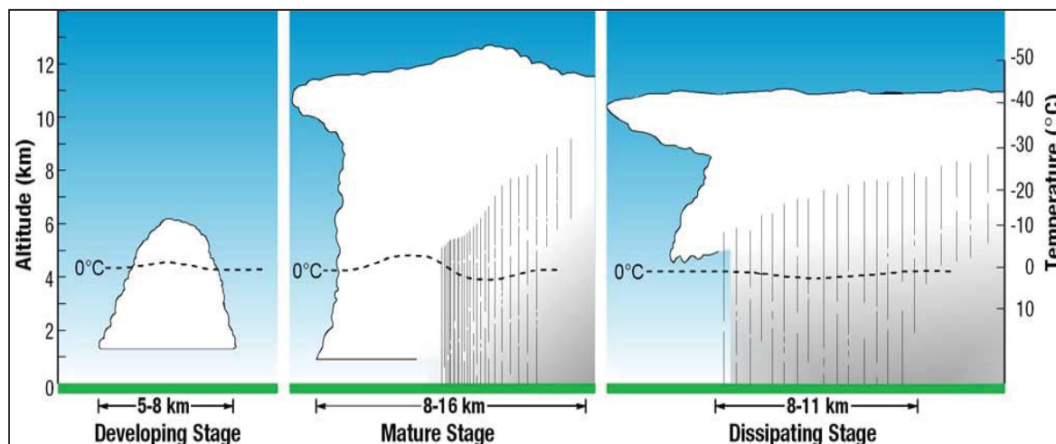
Figure 13-2. The Thunderstorm Life Cycle
