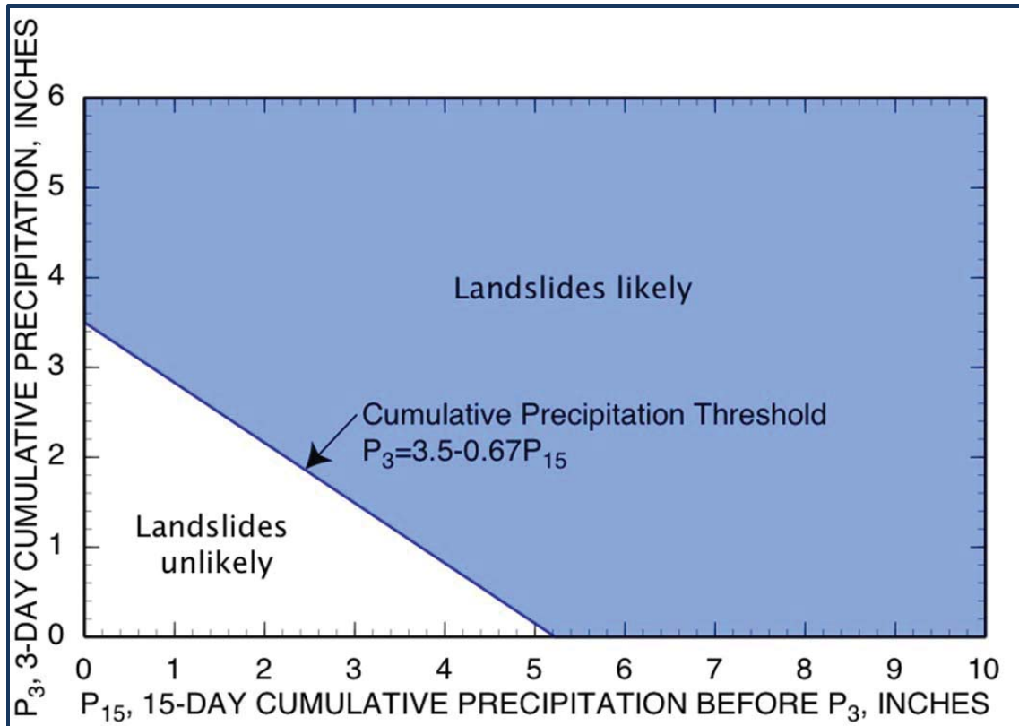
Figure 12-6. Cumulative Precipitation Threshold
