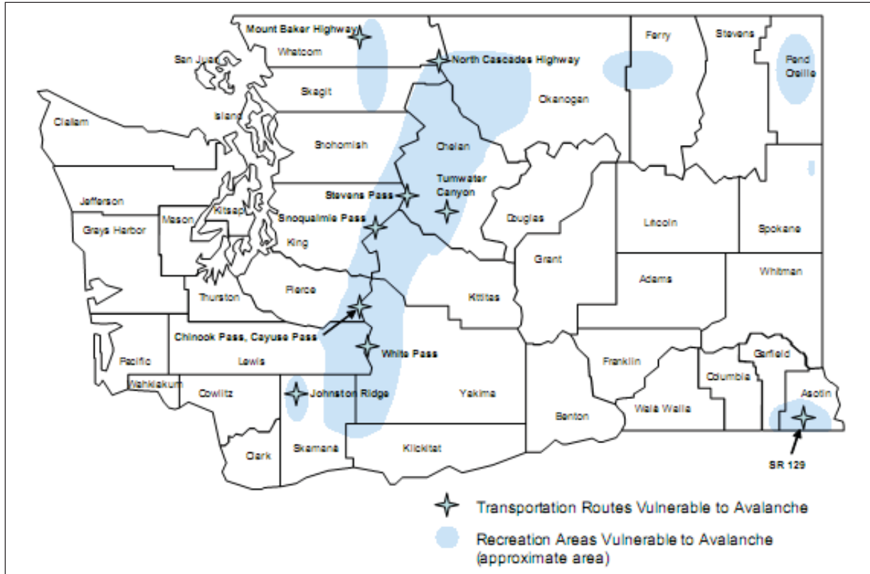
Figure 8-1. Areas Vulnerable to Avalanche
