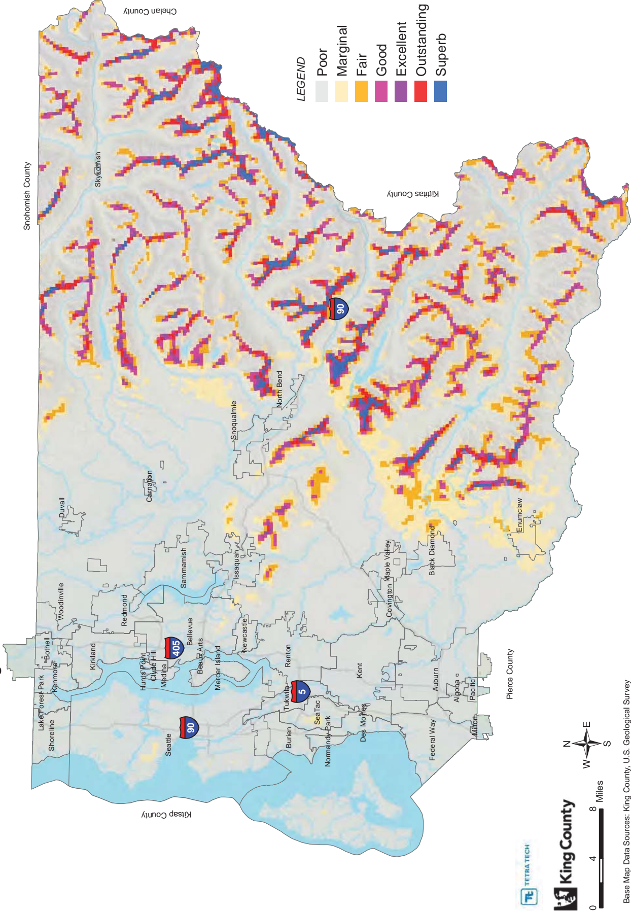
Figure 6-5. Wind Power Class at 50-Meter Height
