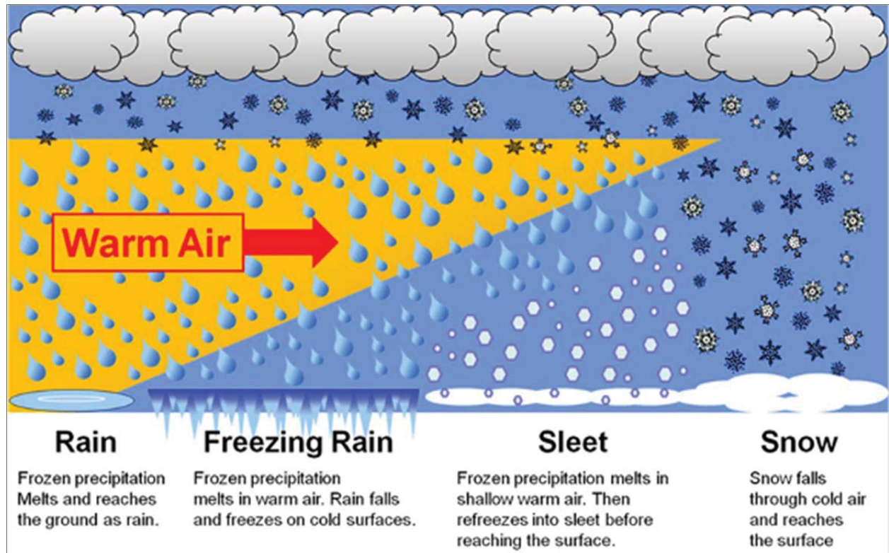
Figure 14-1. The Formation of Different Kinds of Precipitation
