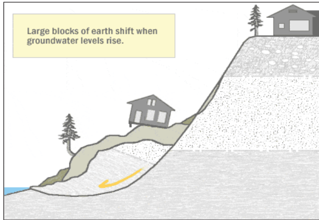
Figure 12-1. Deep Seated Slide
