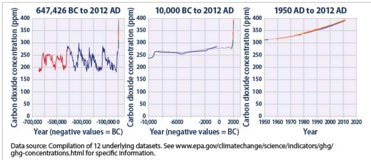
Figure 7-1. Global Carbon Dioxide Concentrations Over Time
