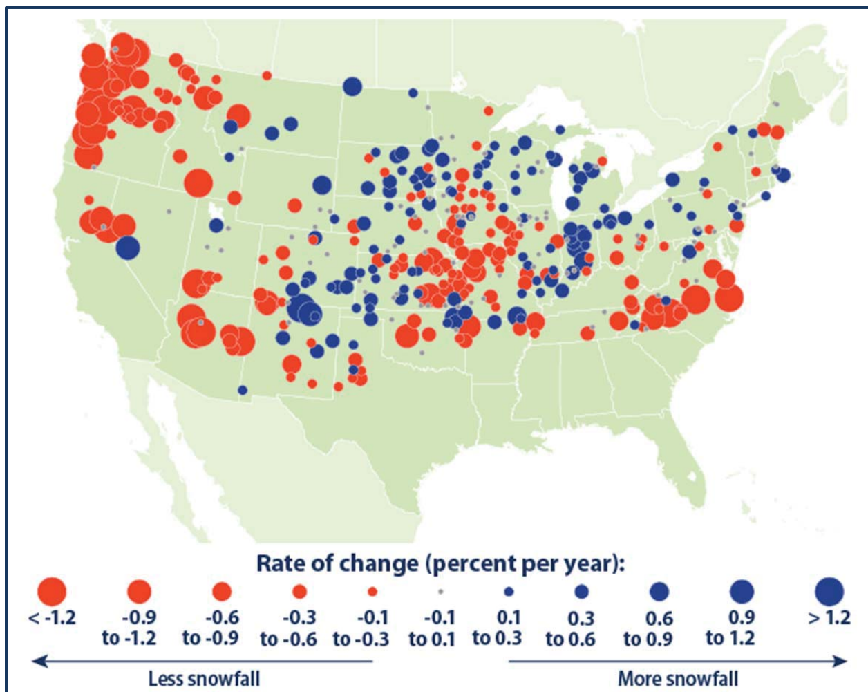
Figure 7-3. Change in snowfall, 1930-2007
