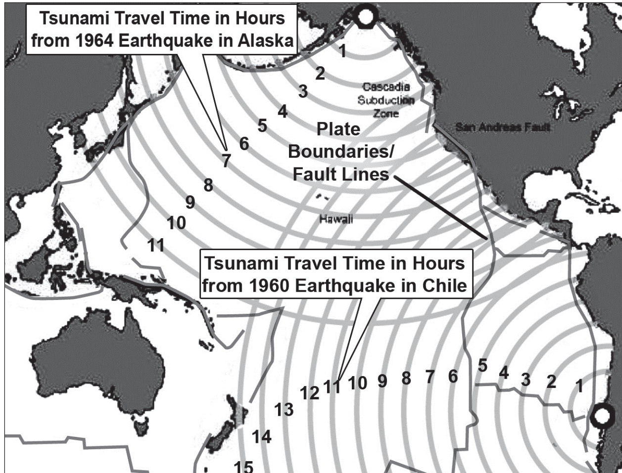
Figure 15-1. Potential Tsunami Travel Times in the Pacific Ocean
