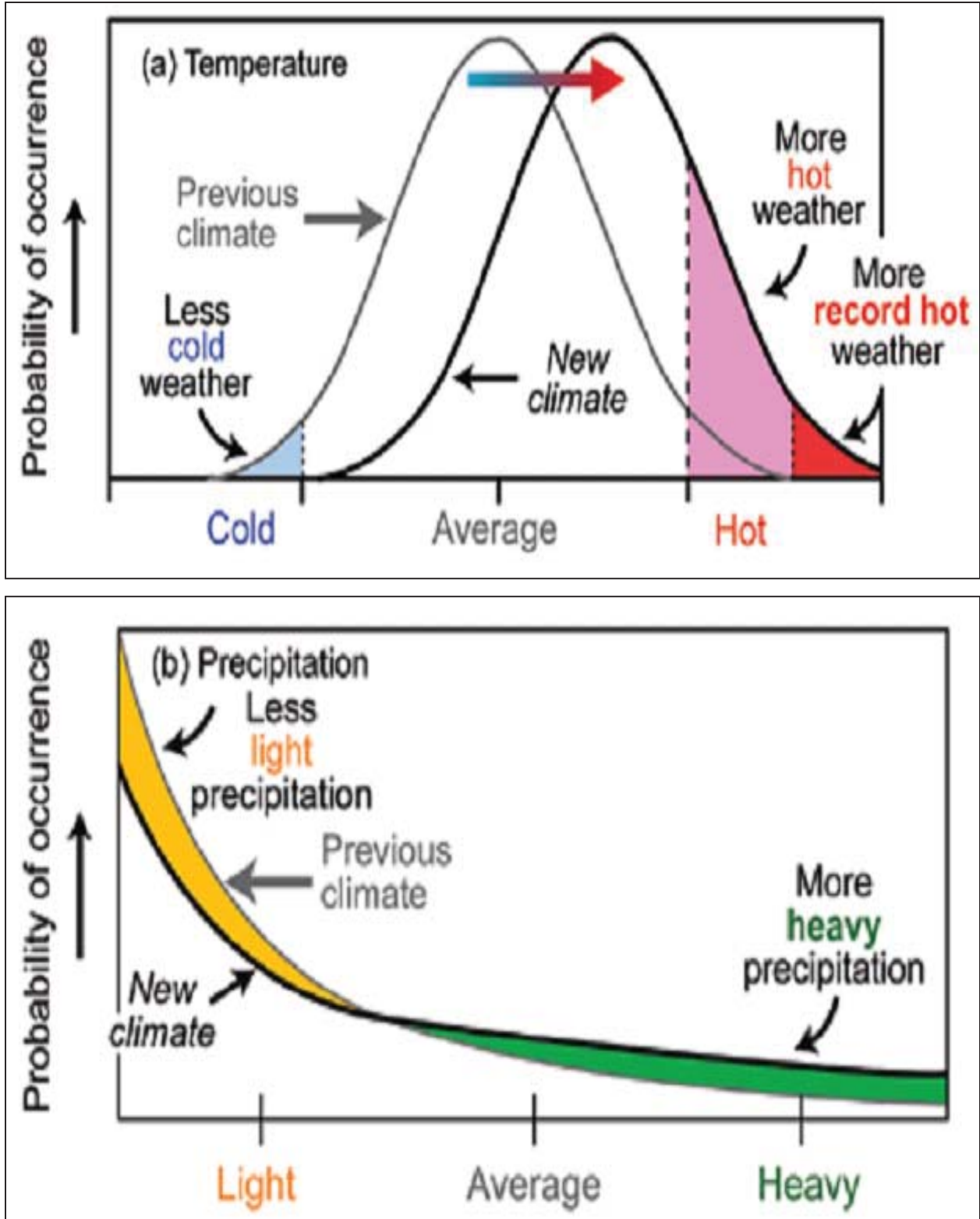
Figure 7-2. Severe Weather Probabilities in Warmer Climates
