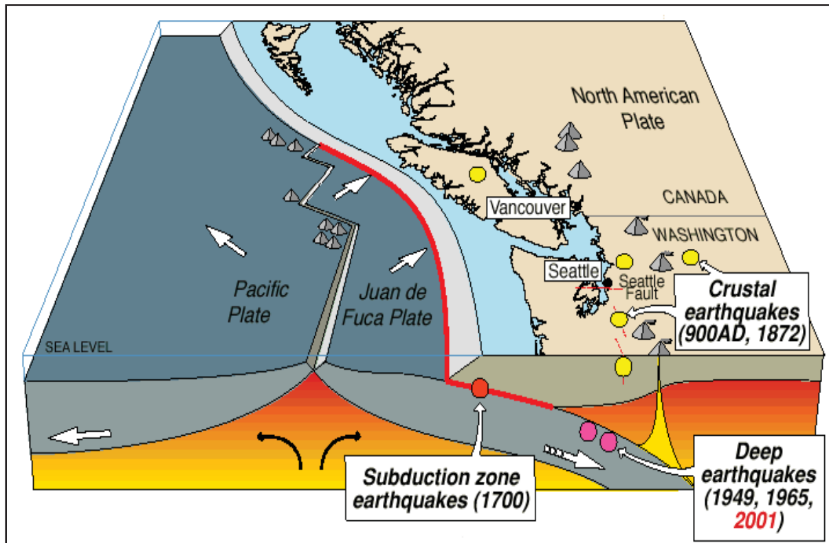
Figure 10-1. Earthquake Types in the Pacific Northwest
