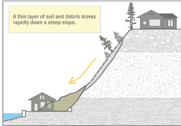
Figure 12-2. Shallow Colluvial Slide
