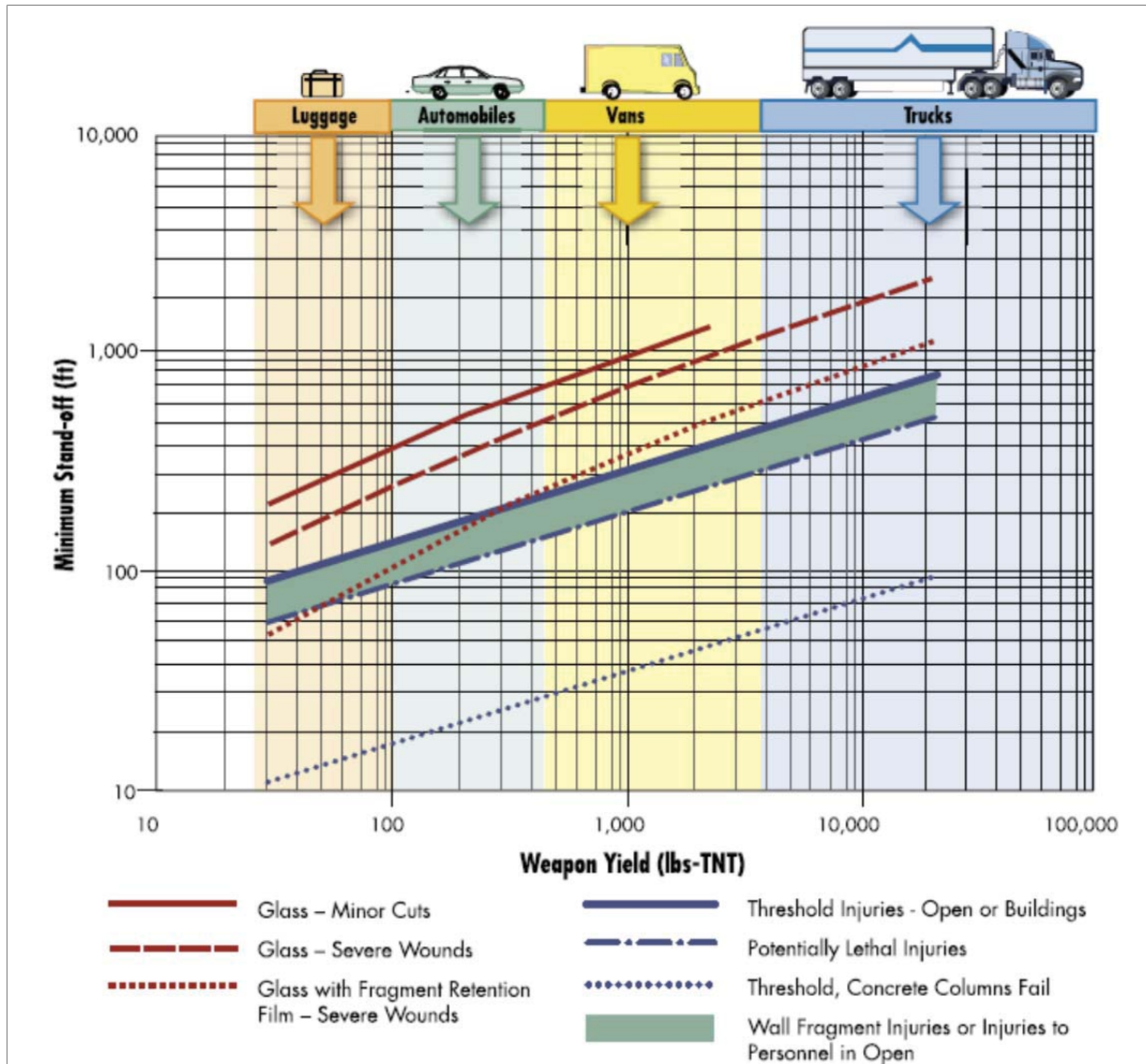
Figure 18-1. Damage Potential from Explosives Based on Delivery Vehicle
