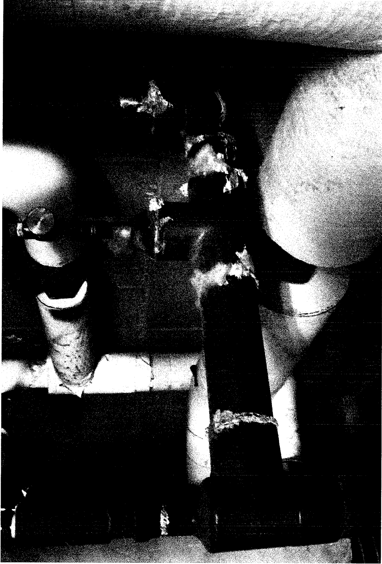
P-2 Pipe At Water Heater Crystalline substance is a salt-like structure. Fuzzy material is leftover fiberglass insulation.
