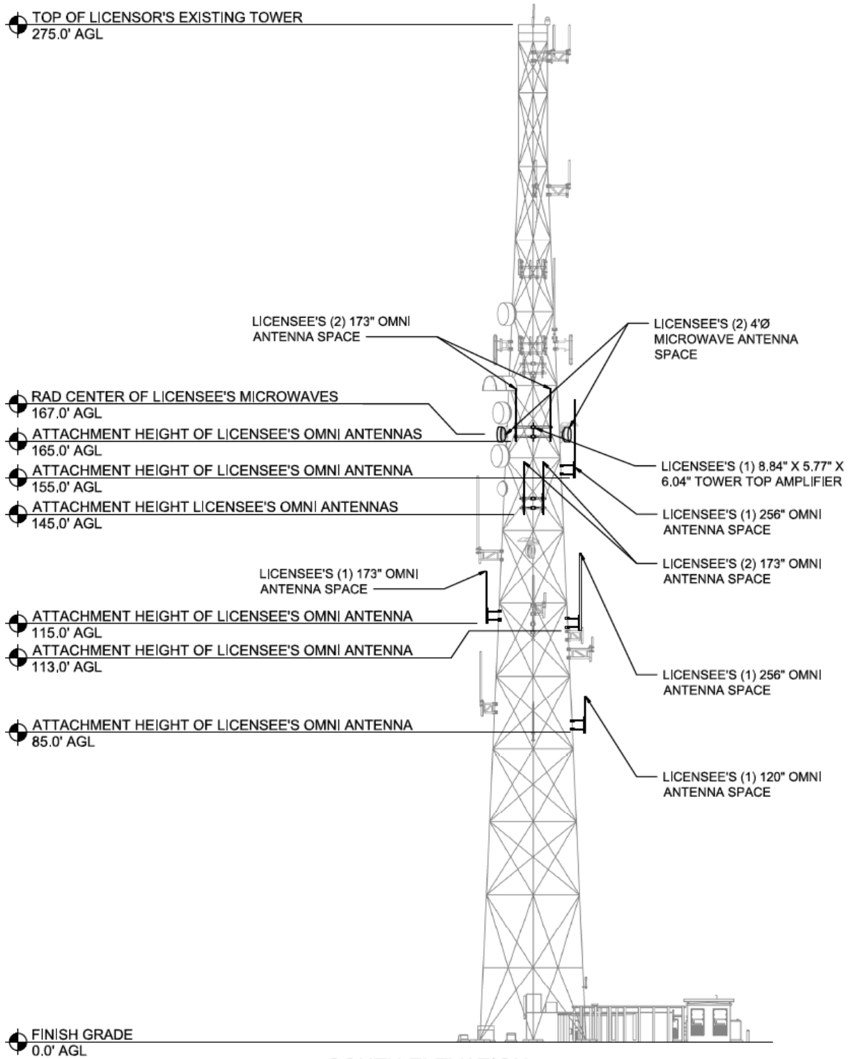
SOUTH ELEVATION
